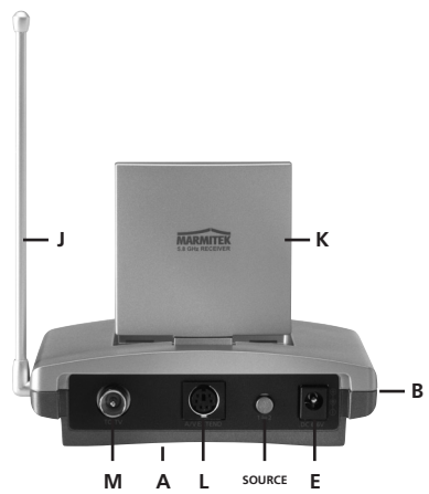
Figure 4 A/V RECEIVER
