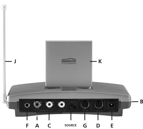
Figure 3 A/V TRANSMITTER
